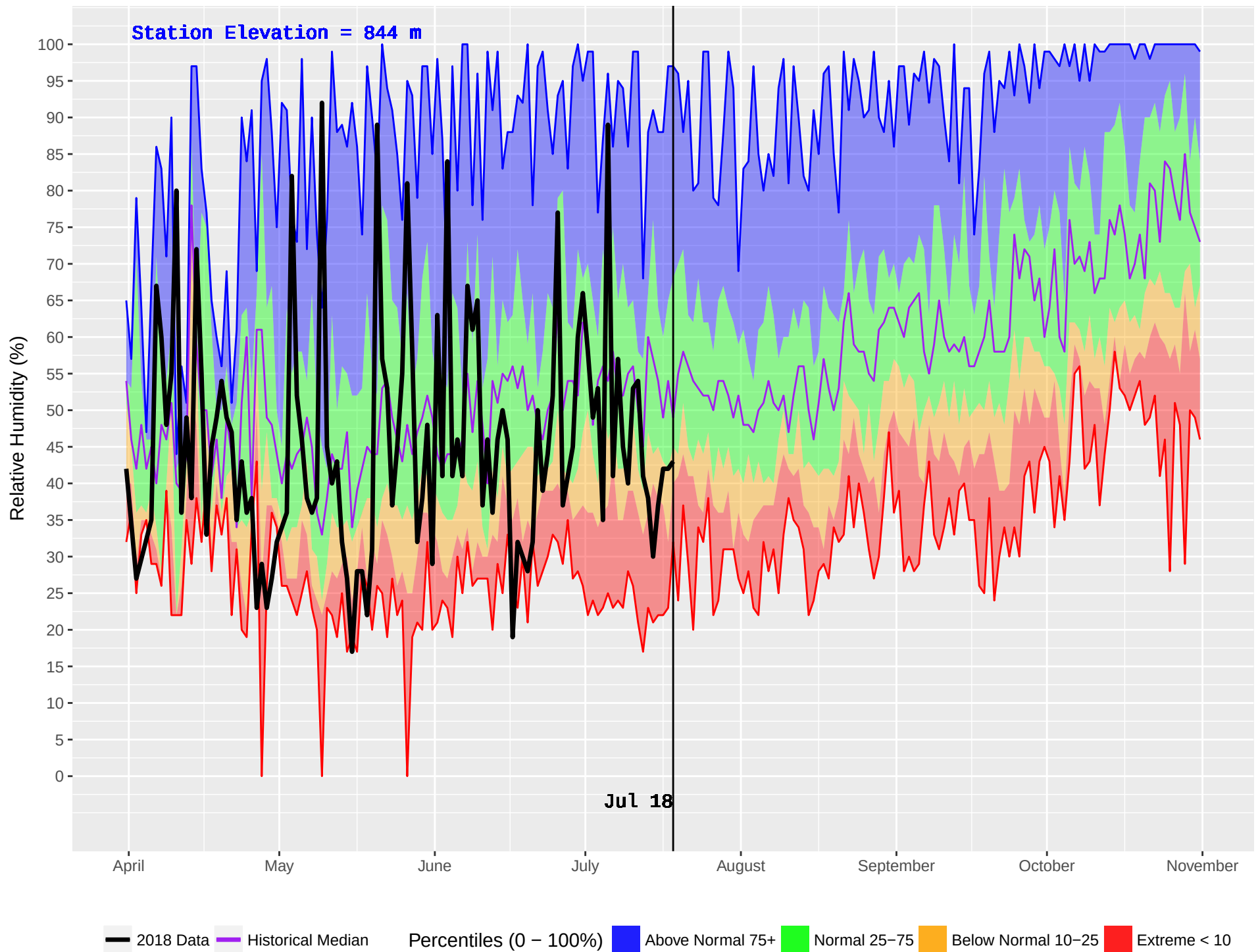
GANOKWA (182) : Historical (1993–2016) and Current (2018) Daily Relative Humidity
