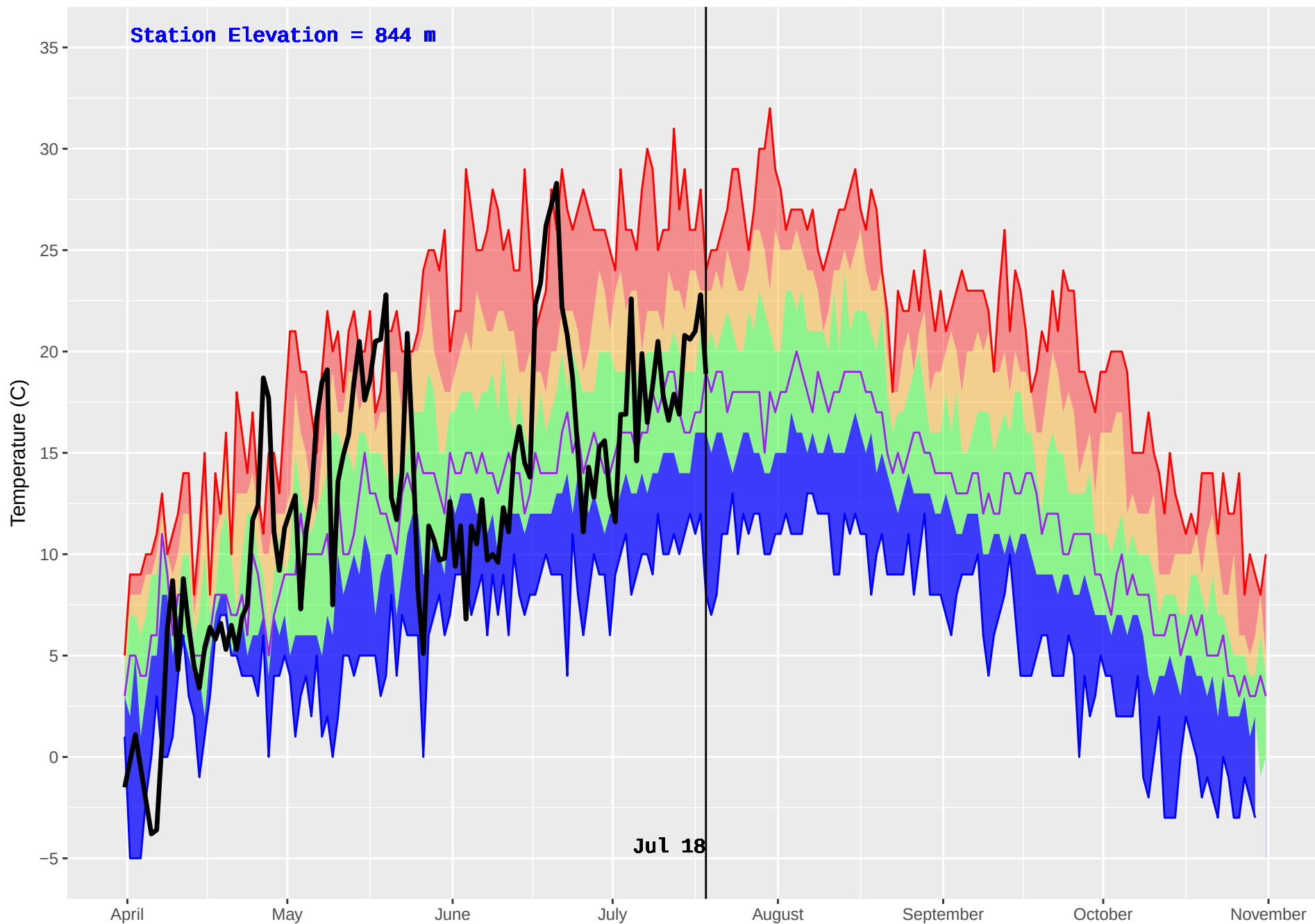
GANOKWA (182) : Historical (1993–2016) and Current (2018) Daily Temperature
