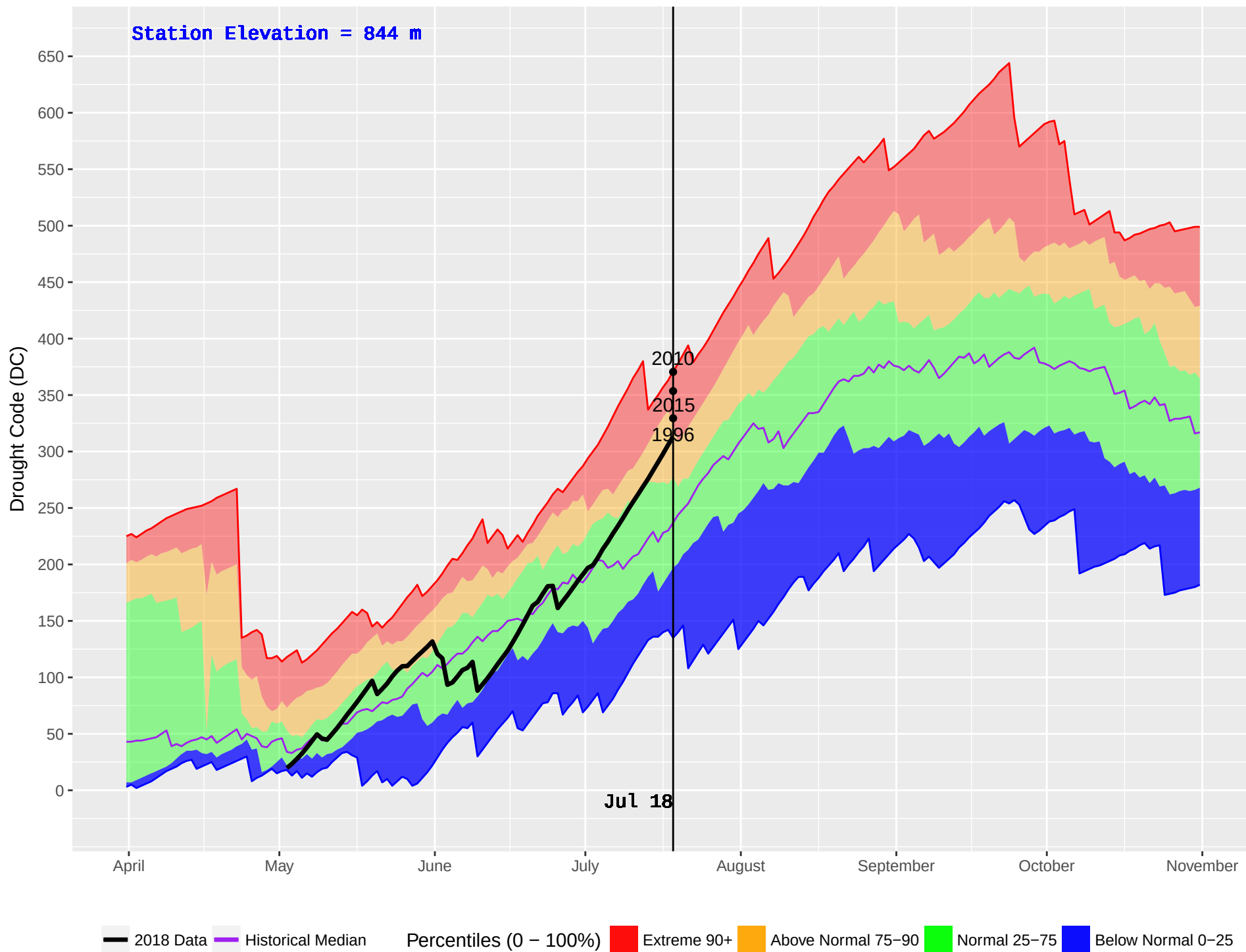
GANOKWA (182) : Historical (1993–2016) and Current (2018) Daily Drought Code (DC)
