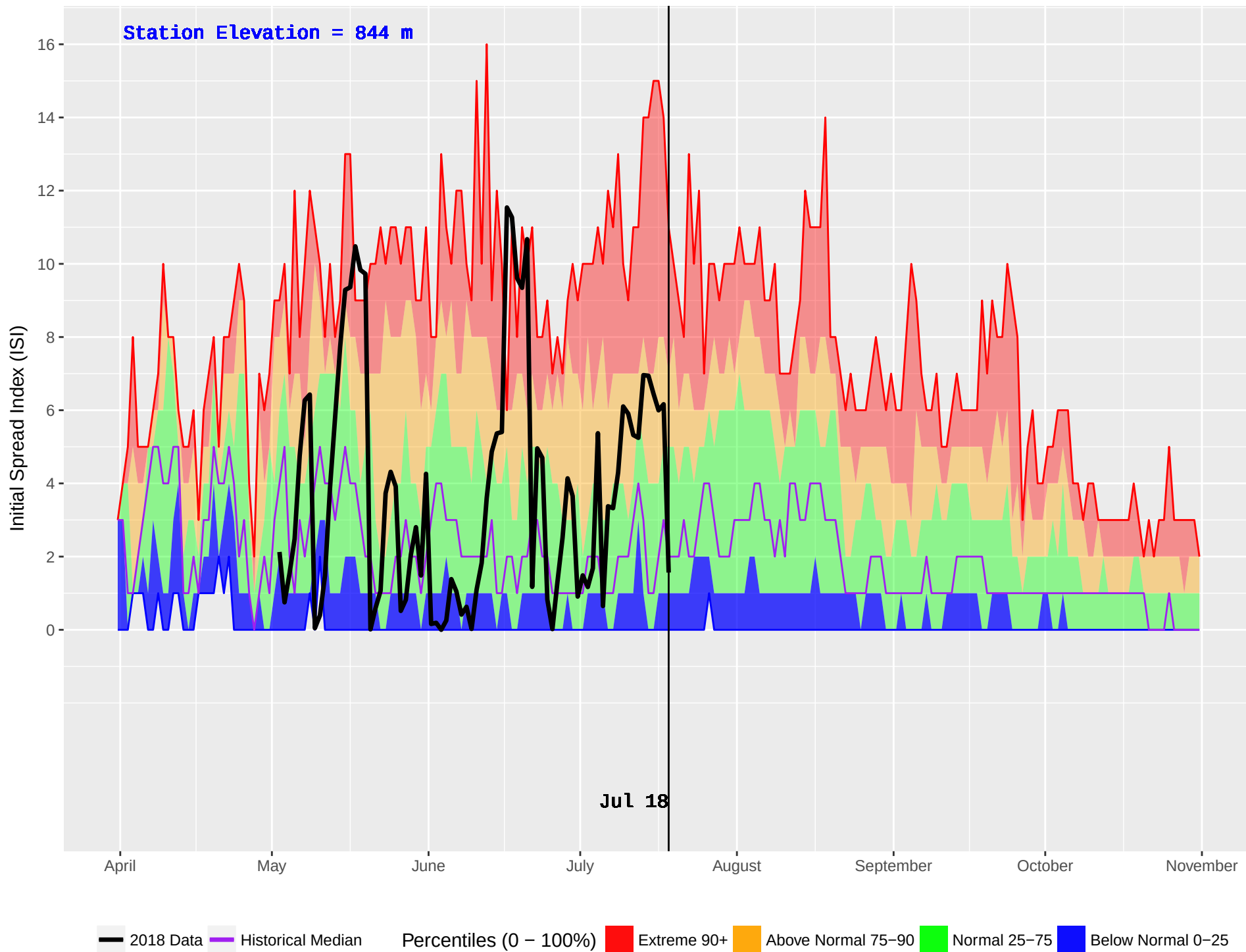
GANOKWA (182) : Historical (1993–2016) and Current (2018) Daily Initial Spread Index (ISI)
