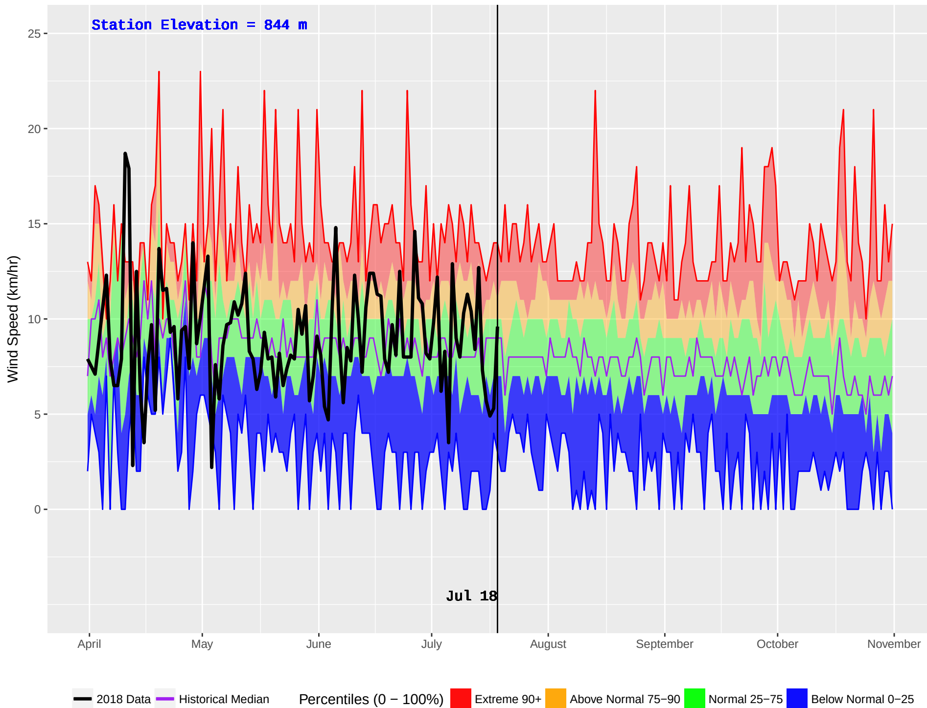
GANOKWA (182) : Historical (1993–2016) and Current (2018) Daily Wind Speed
